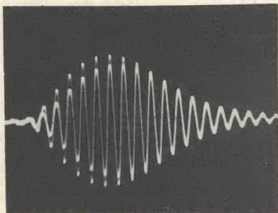
FIG. 4. Oscilloscope display of echoes 2 and 3 from Fig. 2 properly overlapped with respect to "in-phase" condition. The delay time between these two echoes is 2 \mu sec. The carrier frequency is 20 MHz.
